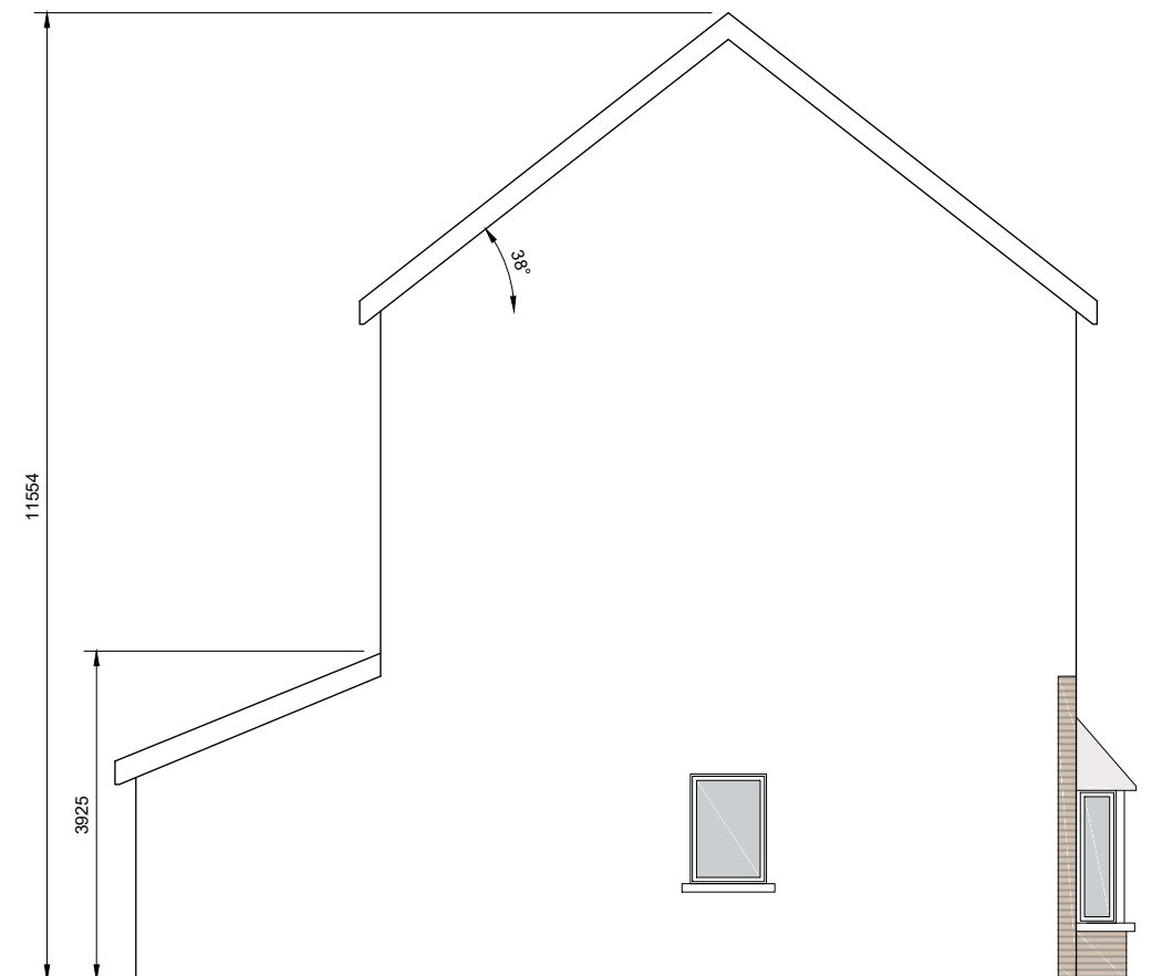
GABLE ELEVATION
